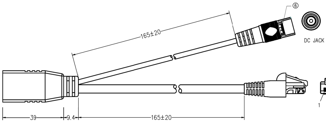
RJ45 JACK
